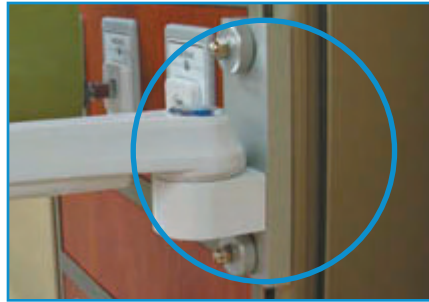
SSM Monitor Arm mounted directly to the vertical headwall
